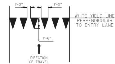
YIELD LINE DETAIL
