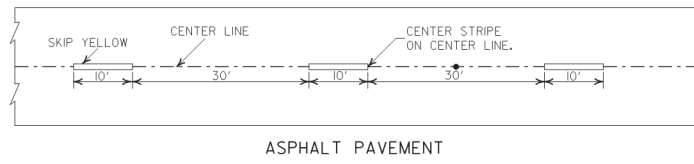
ASPHALT PAVEMENT
