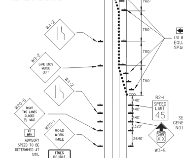
(D) TYPICAL APPLICATION - CLOSING MULTIPLE LANES OF A MULTILANE HIGHWAY.
