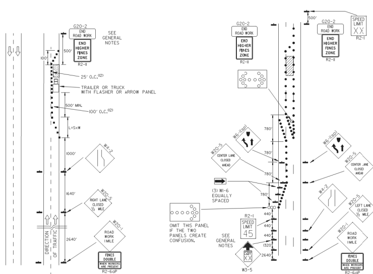
(A) TYPICAL APPLICATION - DAYTIME MAINTENANCE OPERATIONS OF SHORT DURATION ON A 4-LANE DIVIDED ROADWAY WHERE HALF OF THE ROADWAY IS CLOSED.
