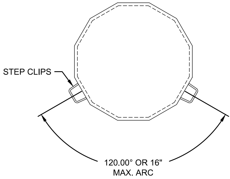
STEP CLIPS DETAIL FOR 3/4" STEP BOLTS
