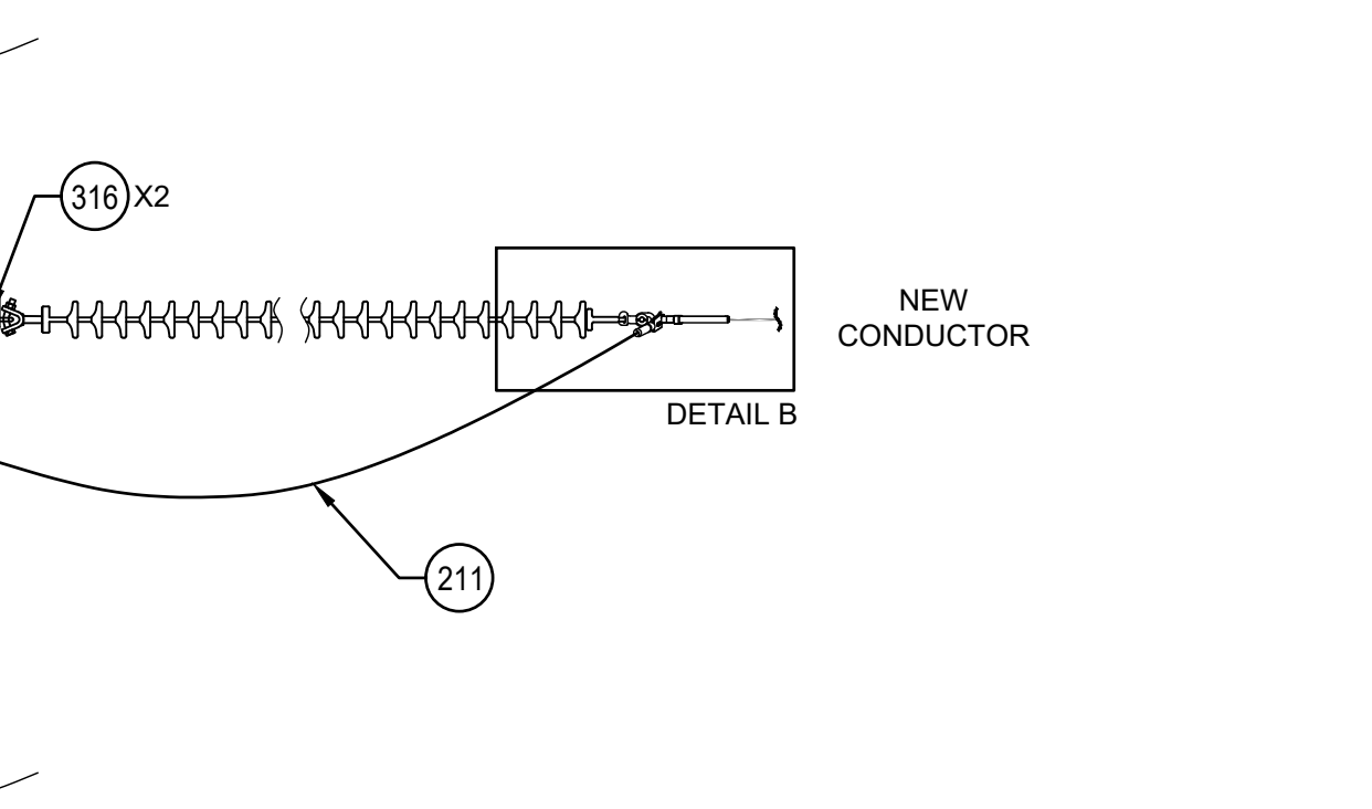
VIEW D-D CONDUCTOR DEADEND ASSEMBLY THREE ASSEMBLIES REQ'D
