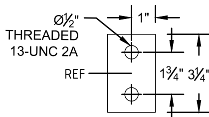
DETAIL G4 2 HOLE THREADED NEMA GROUNDING PLATE
