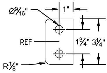
DETAIL G2 2 HOLE NEMA GROUNDING TAB
