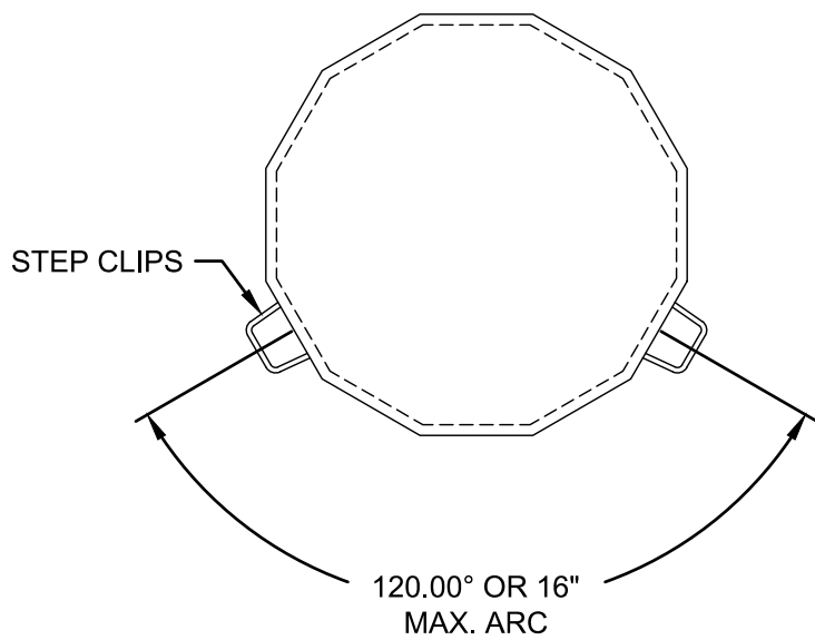
STEP CLIPS DETAIL FOR 3/4" STEP BOLTS
