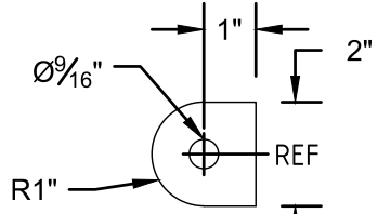
DETAIL G1 GROUNDING TAB
