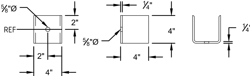
DETAIL F3 OPGW COIL MOUNTING BRACKET (HOLE)
