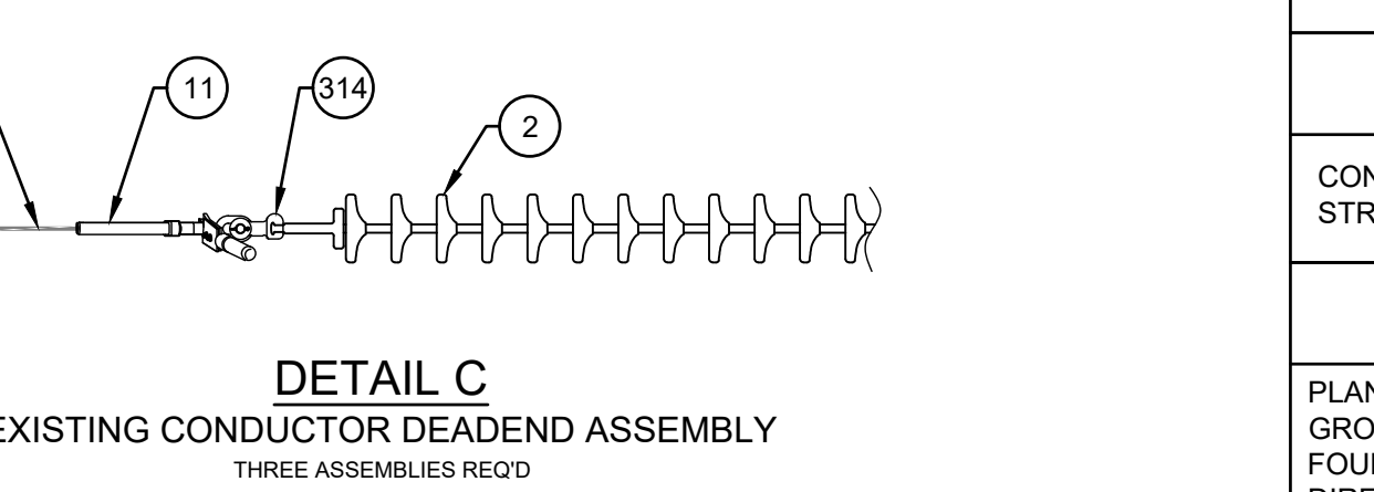
DETAIL C EXISTING CONDUCTOR DEADEND ASSEMBLY THREE ASSEMBLIES REQ'D
