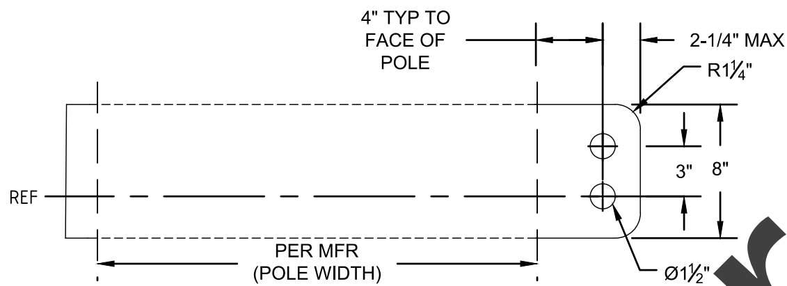
DETAIL V4 ONE-WAY CONDUCTOR VANG
