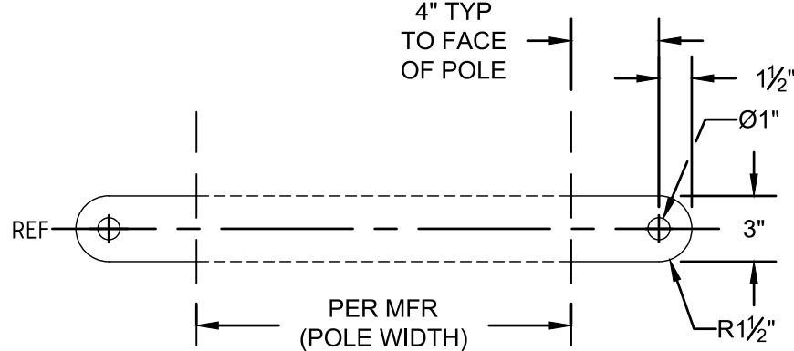
DETAIL V1 TWO-WAY SHIELD/BRACE VANG
