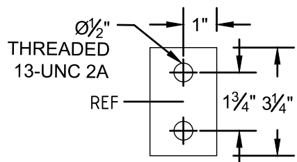
DETAIL G4 2 HOLE THREADED NEMA GROUNDING PLATE
