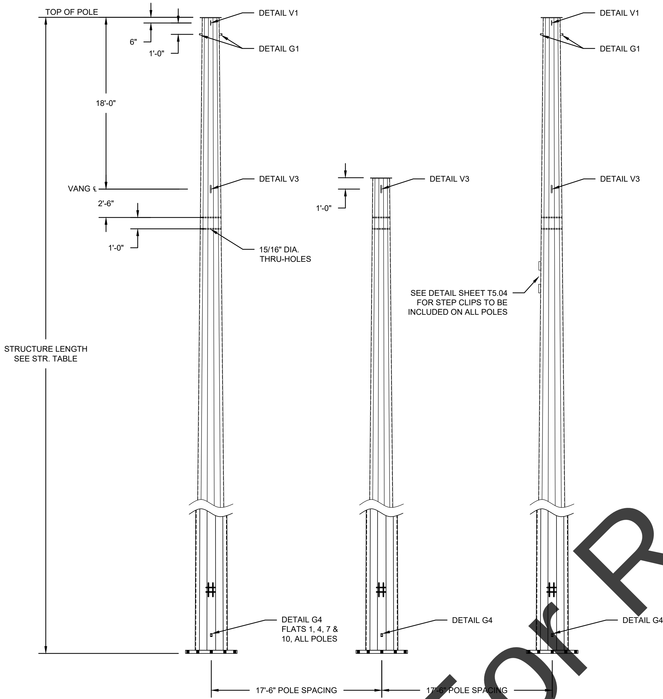
161KV 3-POLE HORIZONTAL DEADEND SMALL ANGLE
