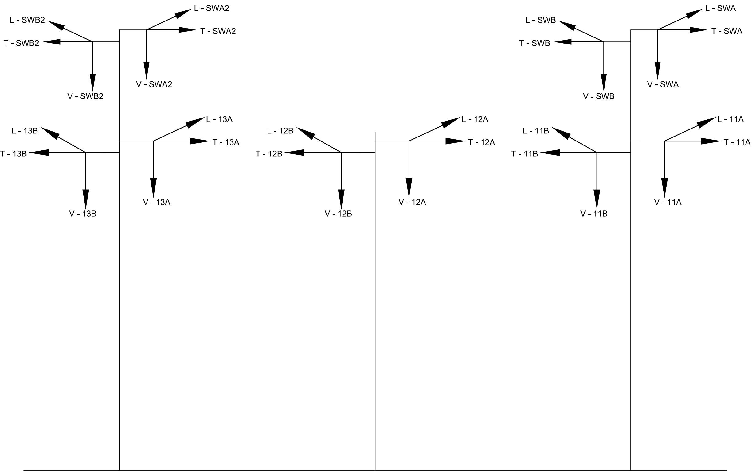
STRUCTURE LOAD TREE CONDUCTOR/SHIELD WIRE LOADS
