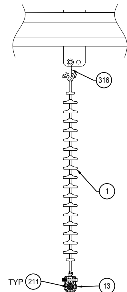
DETAIL C CONDUCTOR SUSPENSION ASSEMBLY THREE ASSEMBLIES REQ'D
