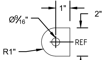
DETAIL G1 GROUNDING TAB
