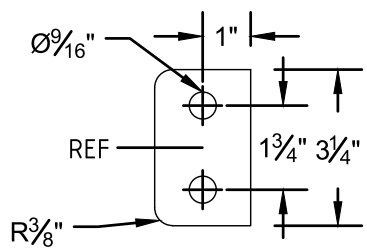
DETAIL G2 2 HOLE NEMA GROUNDING TAB
