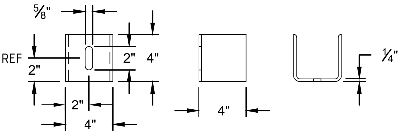
DETAIL F4 OPGW COIL MOUNTING BRACKET (SLOTTED)
