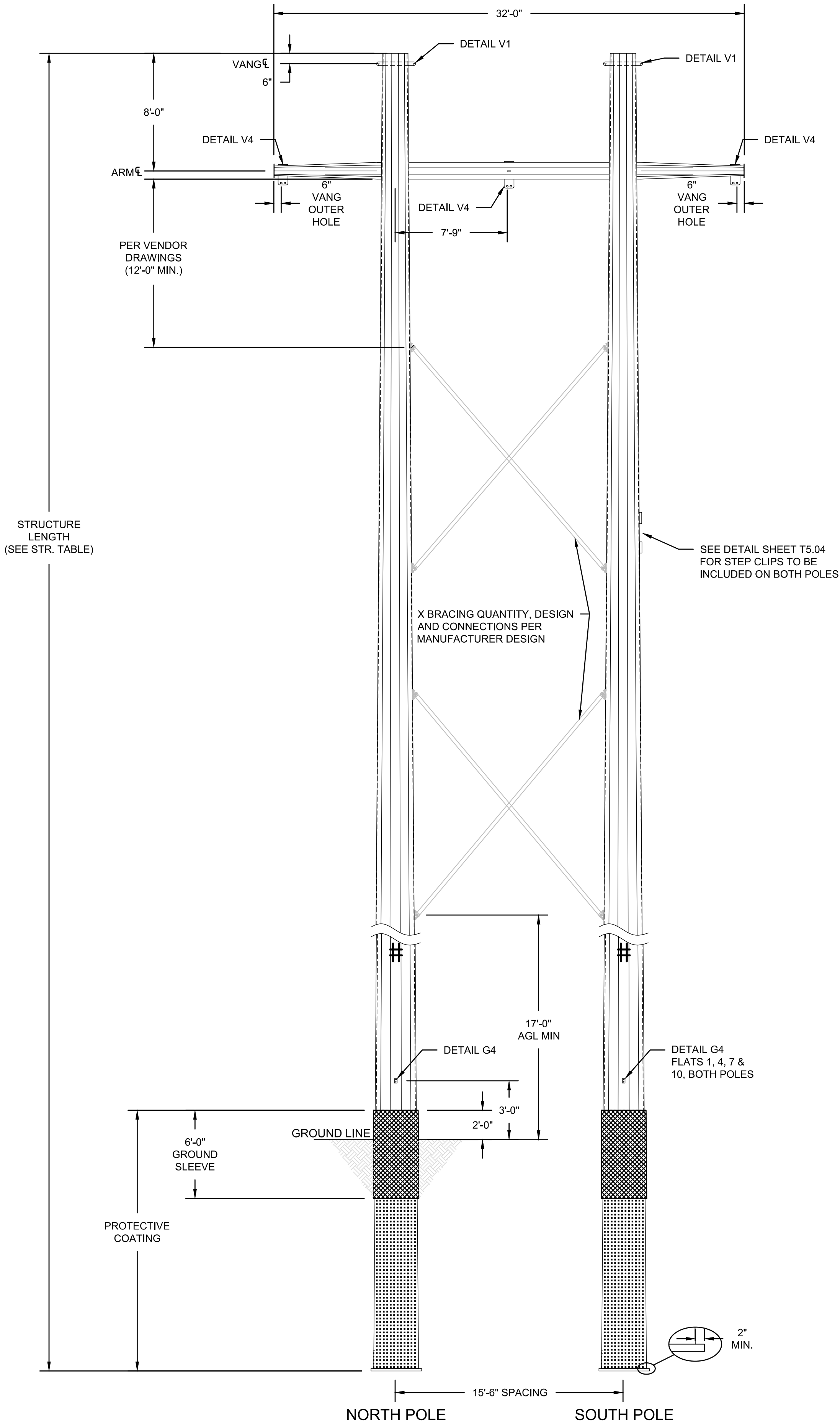
161kV HORIZONTAL TANGENT STRUCTURE SHOWN AT ZERO LINE ANGLE FOR CLARITY
