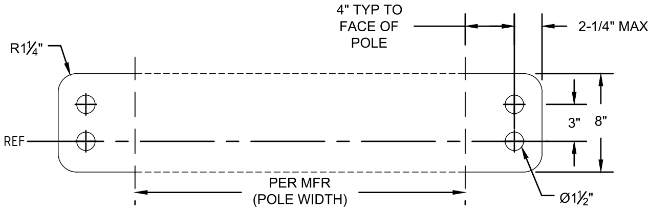
DETAIL V3 TWO-WAY CONDUCTOR VANG
