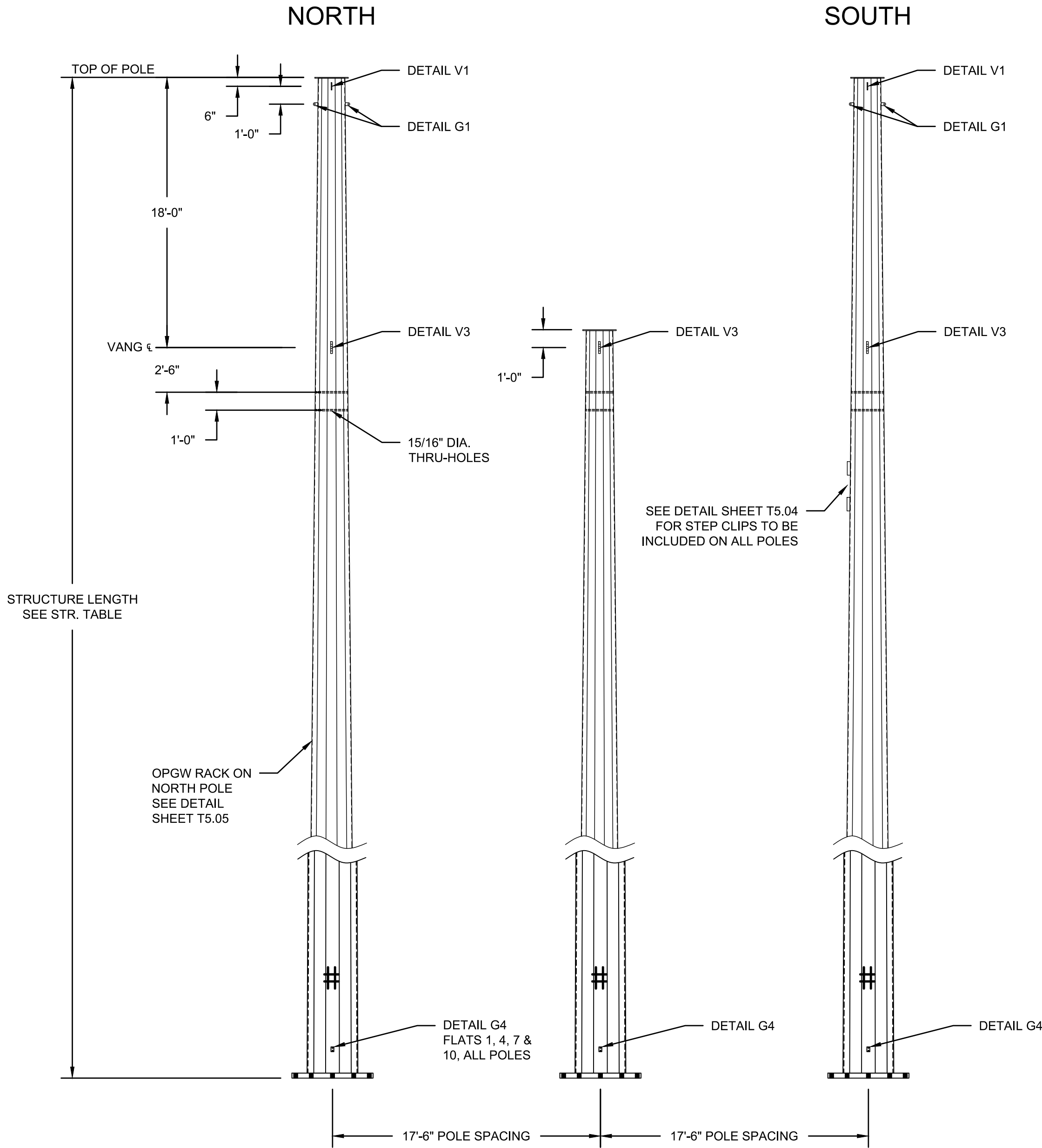
161KV 3-POLE HORIZONTAL DEADEND SMALL ANGLE
