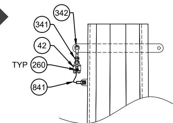
DETAIL A OPGW SUSPENSION ASSEMBLY
