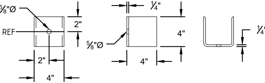
DETAIL F3 OPGW COIL MOUNTING BRACKET (HOLE)
