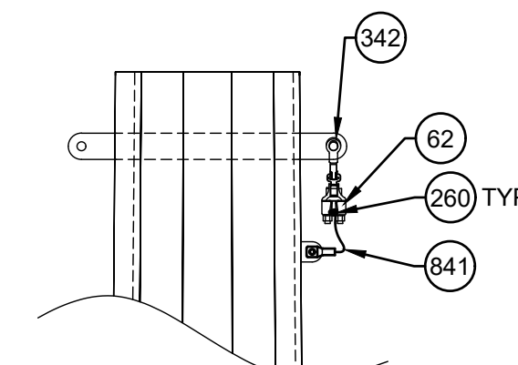
DETAIL B OHGW SUSPENSION ASSEMBLY
