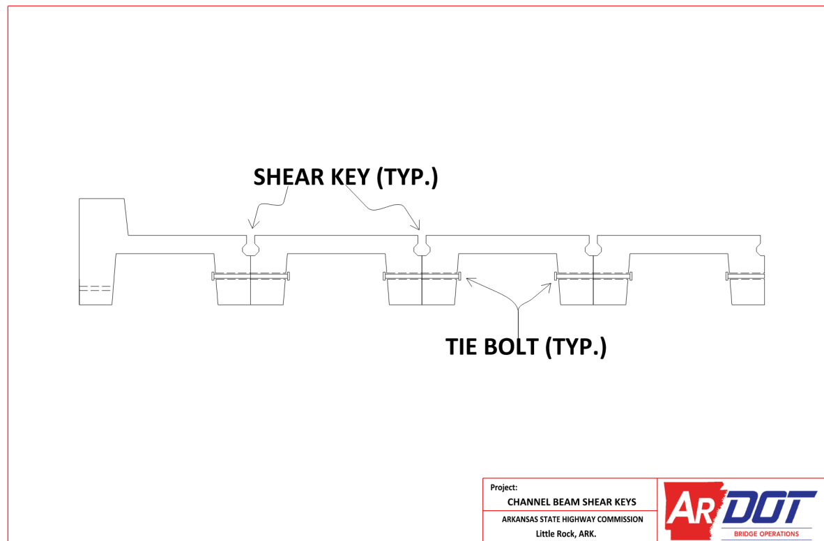
Figure 10. Channel Beams
