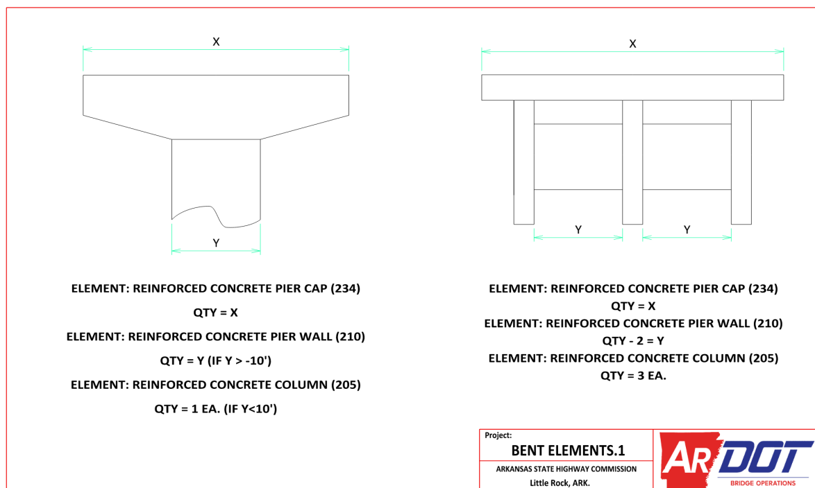
Figure 14. Bent Details 1
