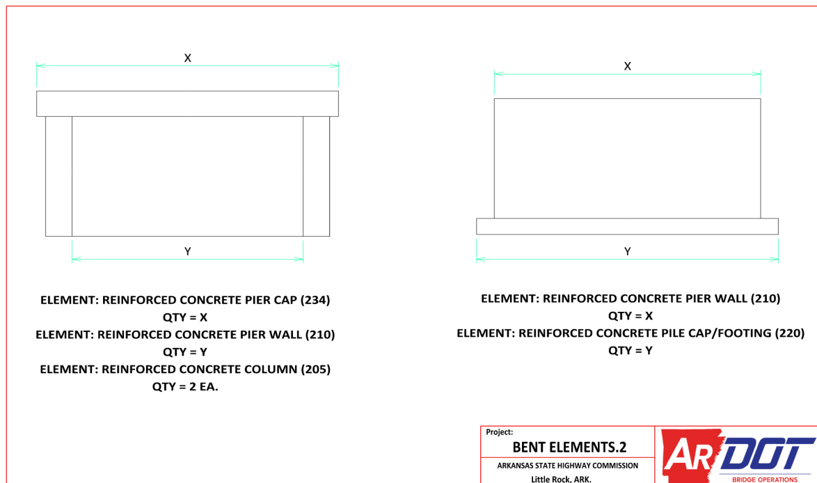
Figure 15. Bent Details 2
