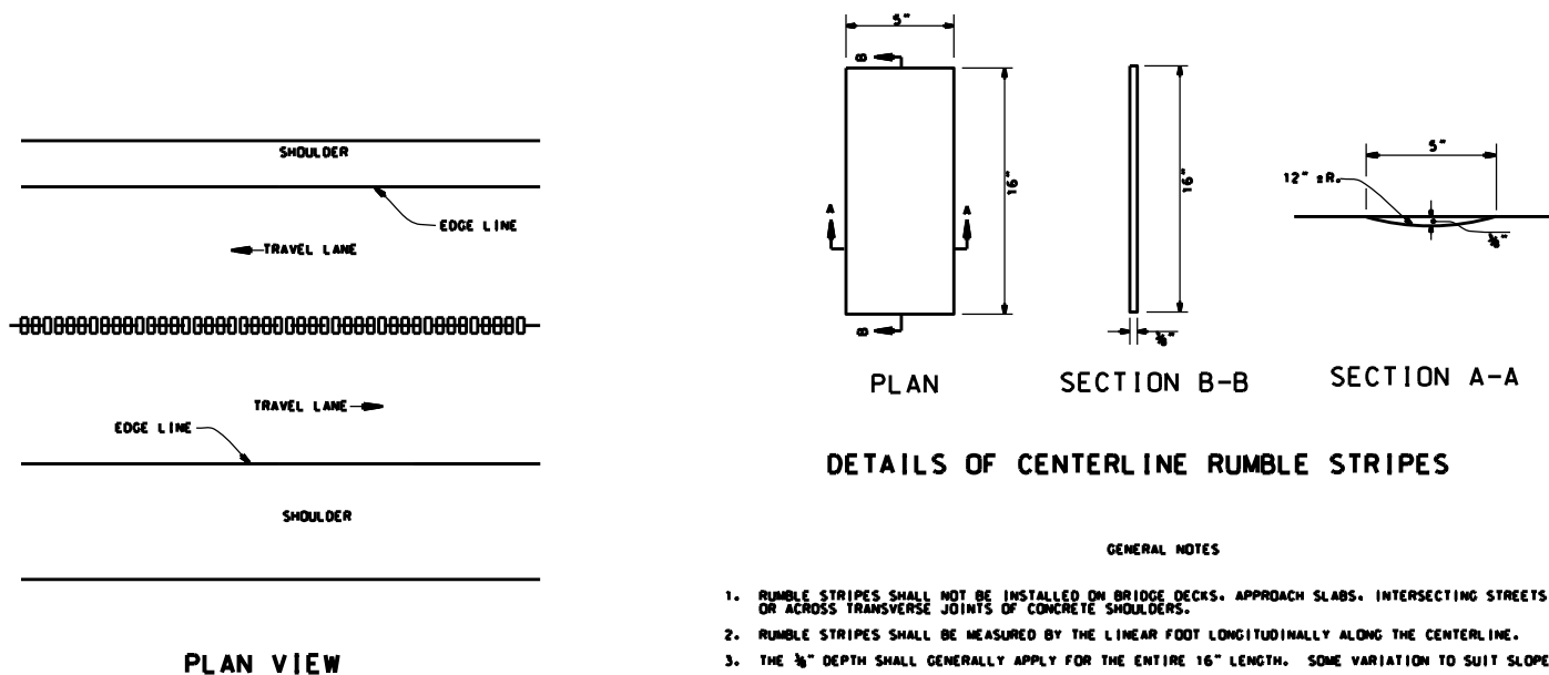
LOCATION PLAN OF CENTERLINE RUMBLE STRIPES
