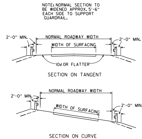
DETAILS SHOWING POSITION OF GUARDRAIL ON HIGHWAY
