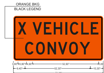
WZ-2 SIGN
