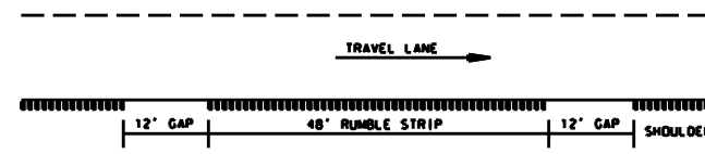
DETAIL FOR GAP PATTERN RUMBLE STRIP
