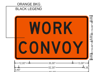
WZ-3 SIGN
