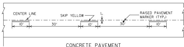
CONCRETE PAVEMENT
