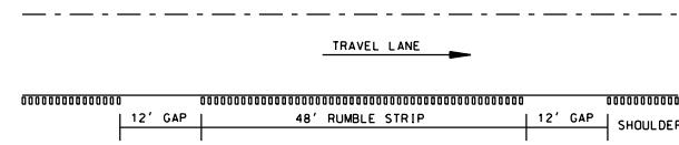
DETAIL FOR GAP PATTERN RUMBLE STRIP
