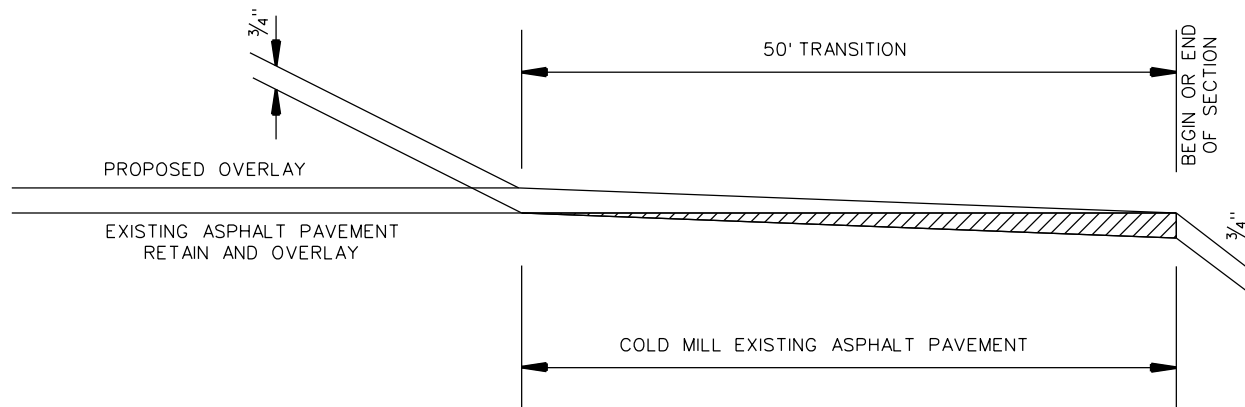
DETAIL FOR TRANSITIONS – ULTRATHIN BONDED WEARING COURSE ( \frac{3}{4}" TYPE C)
