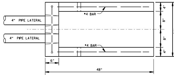
PLAN VIEW
