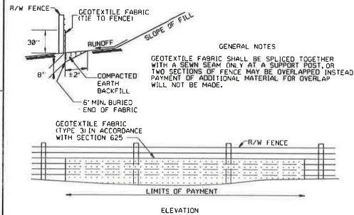
SILTS FENCE ON R/W FENCE (E-4)
