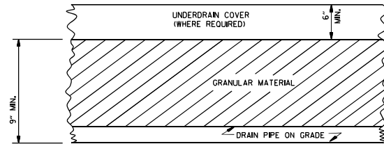
DETAILS OF PIPE UNDERDRAIN
