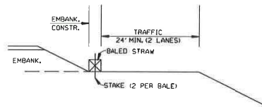
BALED STRAW FILTER BARRIER (E-2)
