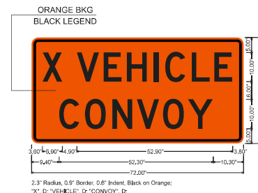
WZ-2 SIGN
