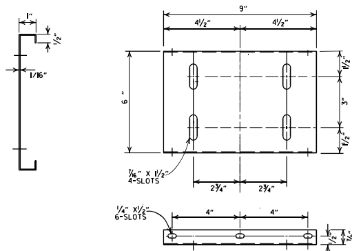
PLATFORM
