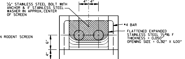
FRONT VIEW (DETAIL OF RODENT SCREEN)
