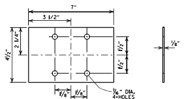
ANTI-TWIST PLATE
