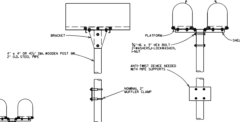
DOUBLE INSTALLATION
