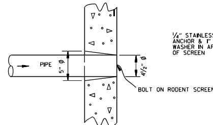
DETAIL OF HOLE FOR 4" PIPE
