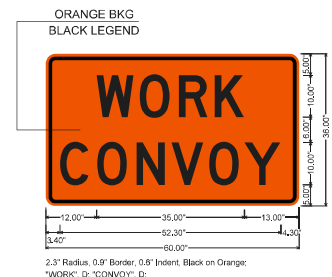
WZ-3 SIGN
