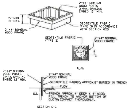
DROP INLET SILTS FENCE (E-7)
