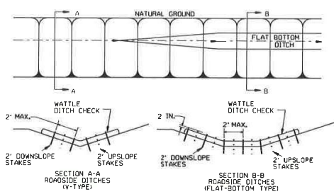
WATTLE DITCH CHECK (E-1)
