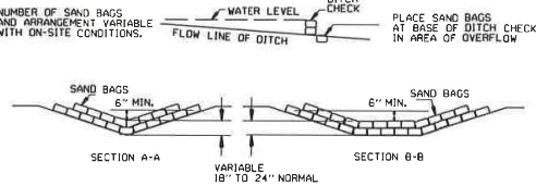
SAND BAG DITCH CHECK (E-5)
