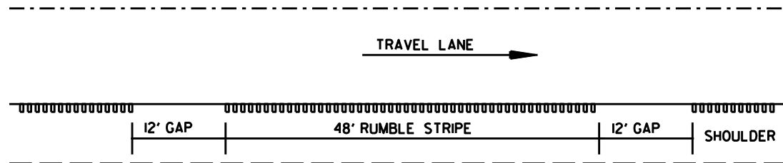
DETAIL FOR RUMBLE STRIPE GAP AT DRIVEWAY TURNOUTS
