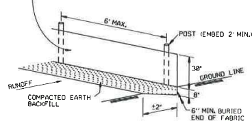
SILTS FENCE (E-11)
