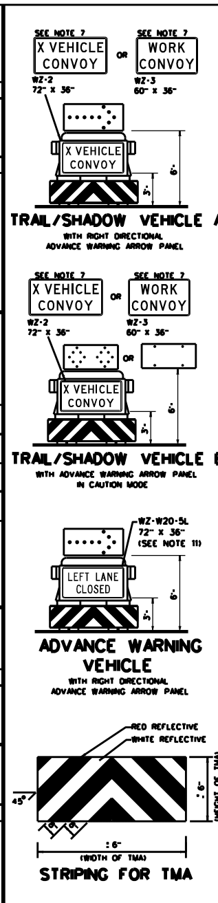
TYPICAL APPLICATION - MOBILE WORK ZONE
