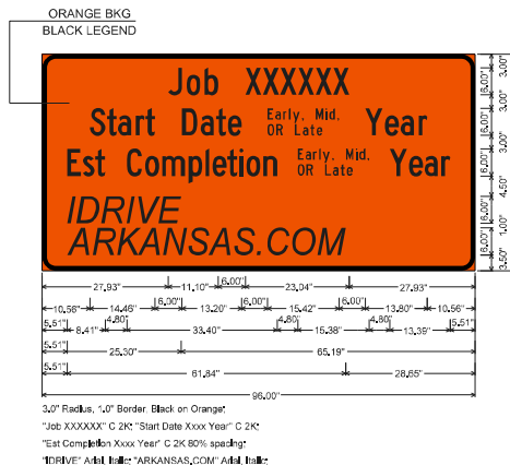
CONSTRUCTION PROJECT INFORMATION SIGN
