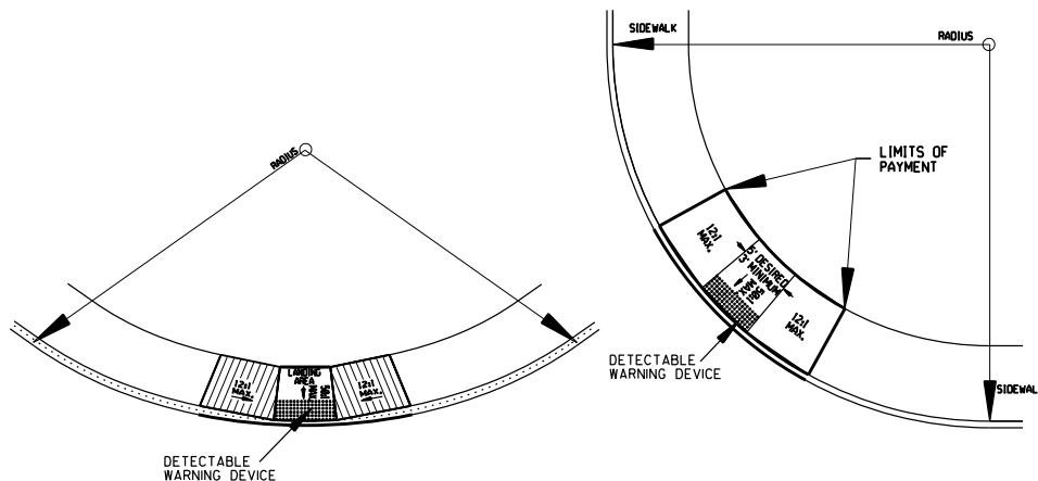
TYPE 6 RAMP
