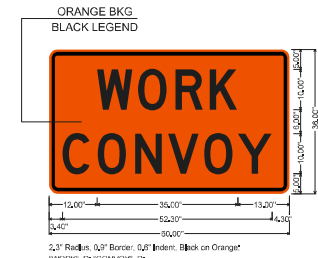
WZ-3 SIGN
