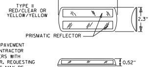
DETAIL OF STANDARD RAISED PAVEMENT MARKERS
