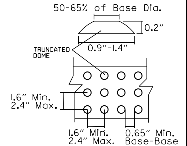
DETECTABLE WARNING DEVICE DETAIL
