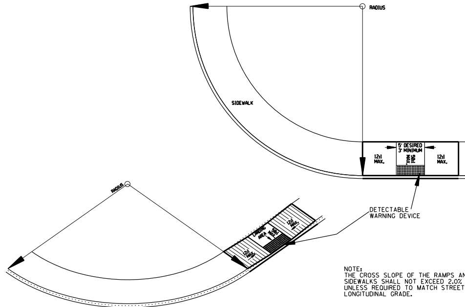
TYPE 5 RAMP
