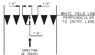
YIELD LINE DETAIL
