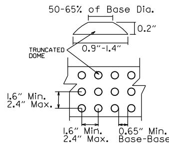
DETECTABLE WARNING DEVICE DETAIL
