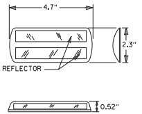
DETAIL OF STANDARD RAISED PAVEMENT MARKERS
