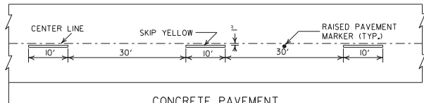
CONCRETE PAVEMENT
