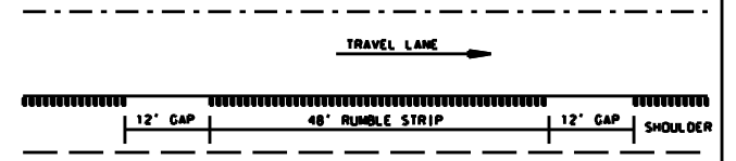
NOTE: GAP PATTERN SHALL BE ADJUSTED BY THE ENGINEER IN THE FIELD ALLOWING FOR DRIVEWAYS TO SERVE AS THE GAP. DETAIL FOR GAP PATTERN RUMBLE STRIP
