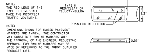
DETAIL OF STANDARD RAISED PAVEMENT MARKERS
