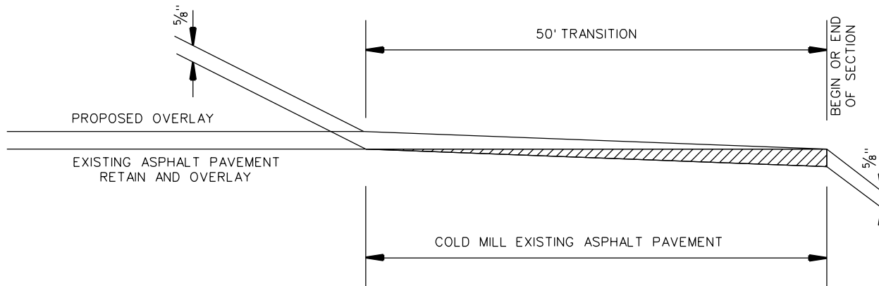
DETAIL FOR TRANSITION - UTBWC MAIN LANES
