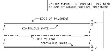
PAVEMENT EDGE LINE MARKING
