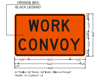
WZ-3 SIGN
