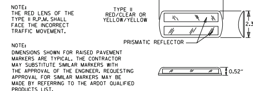
DETAIL OF STANDARD RAISED PAVEMENT MARKERS
