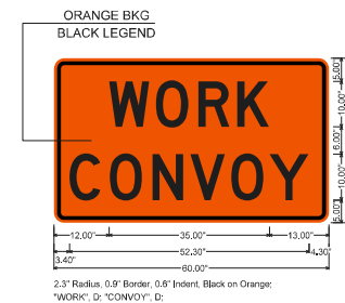
WZ-3 SIGN
