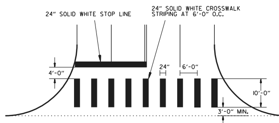
CROSSWALK AND STOP LINE DETAILS
