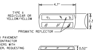
DETAIL OF STANDARD RAISED PAVEMENT MARKERS
