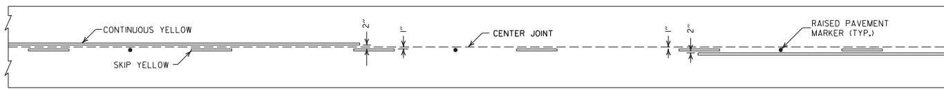
SOLID LINE STRIPING ON CONCRETE PAVEMENT
