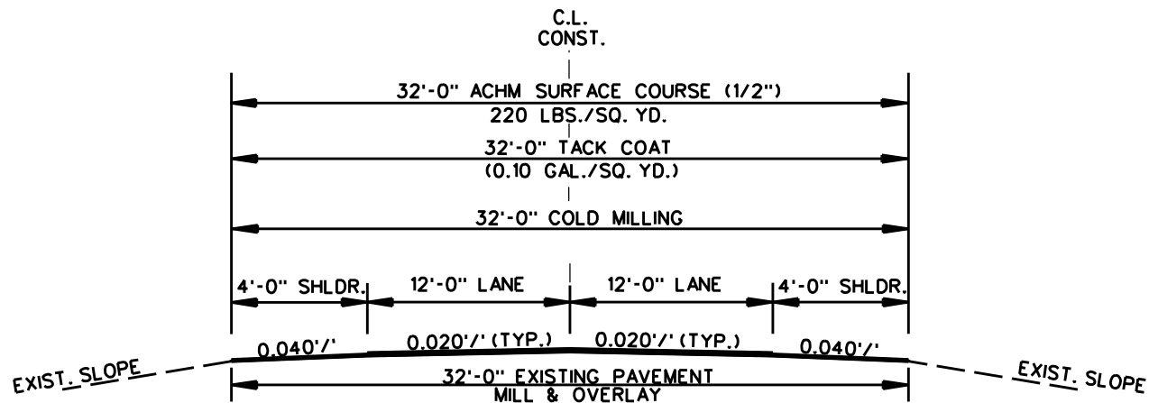
2 LANE OPEN SHOULDER MILL & OVERLAY (4'-0" SHLDR.) LOG MILE 4.430 TO LOG MILE 5.406
