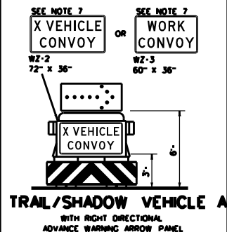
TYPICAL APPLICATION - MOBILE WORK ZONE
