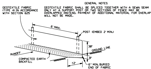
SILT FENCE (E-11)
