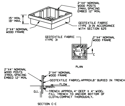
DROP INLET SILT FENCE (E-7)
