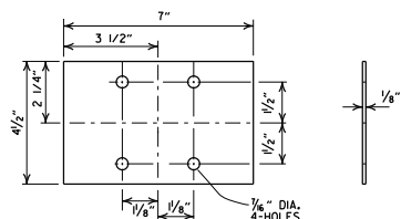
ANTI-TWIST PLATE
