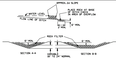
ROCK DITCH CHECK (E-6)
