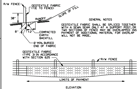
SILT FENCE ON R/W FENCE (E-4)
