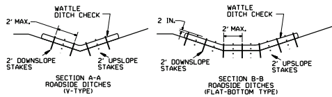
WATTLE DITCH CHECK (E-1)
