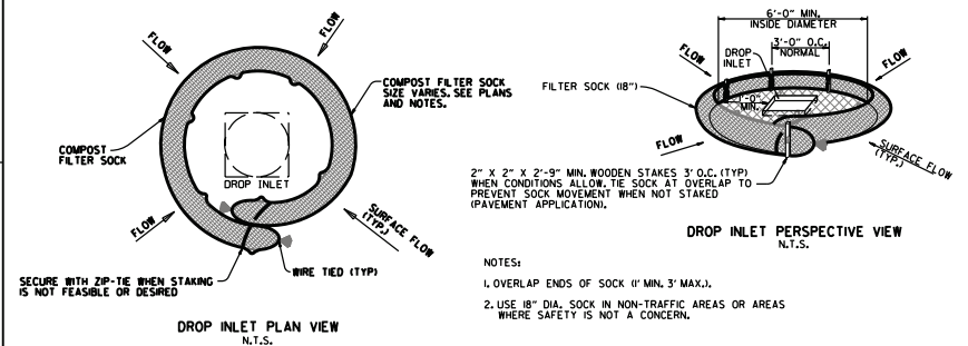
COMPOST FILTER SOCK DROP INLET PROTECTION (E-13)
