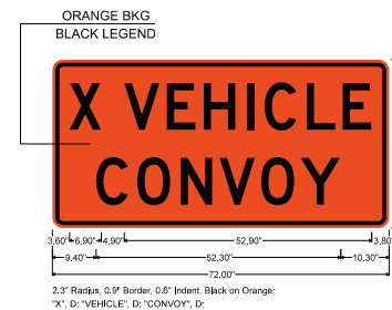
WZ-2 SIGN
