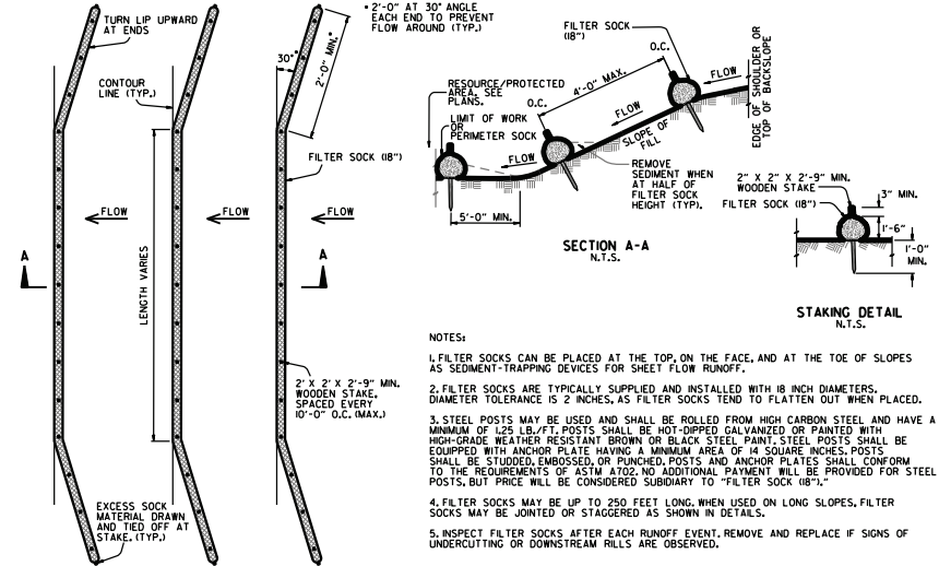
FILTER SOCK ALONG SLOPE (E-3)
