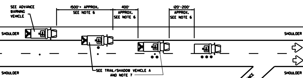
DIVIDED MULTILANE HIGHWAY
