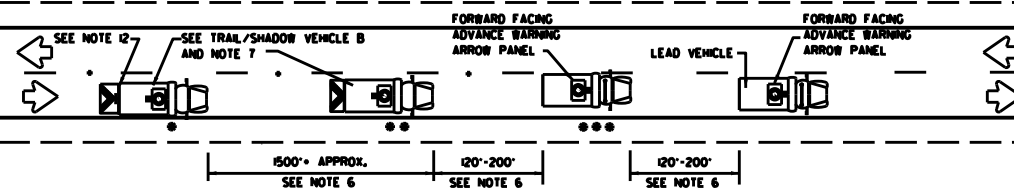
TWO LANE HIGHWAY (WORK ON TRAVEL LANE)
