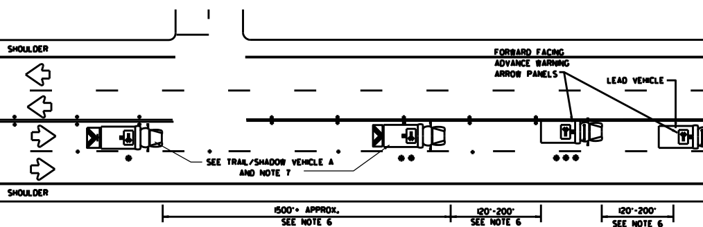
UNDIVIDED MULTILANE HIGHWAY
