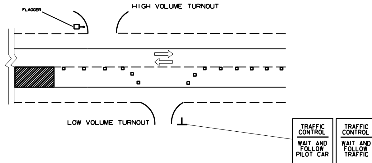
TYPICAL TRAFFIC CONTROL DETAIL FOR COUNTY ROADS AND CITY STREETS.
