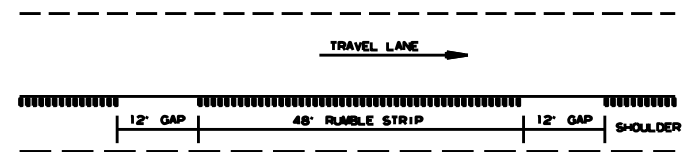
DETAIL FOR GAP PATTERN RUMBLE STRIP
