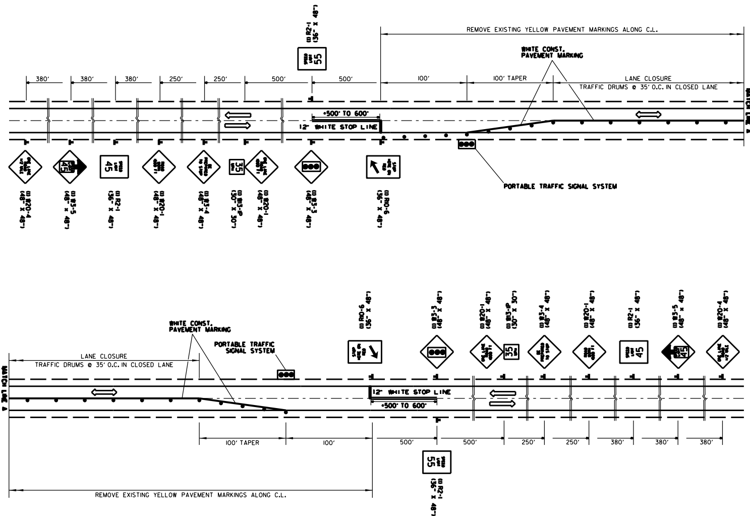
LANE CLOSURE WITH PORTABLE TRAFFIC SIGNAL SYSTEM & TRAFFIC DRUMS
