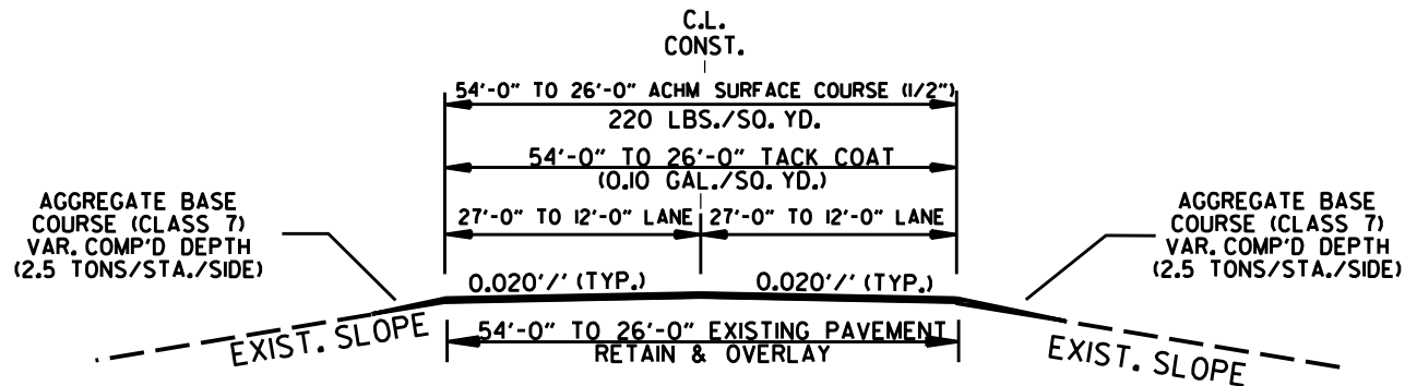
2 LANE OPEN SHOULDER OVERLAY LOG MILE 0.720 TO LOG MILE 0.755
