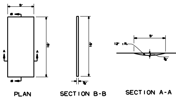
DETAILS OF CENTERLINE RUMBLE STRIPES
