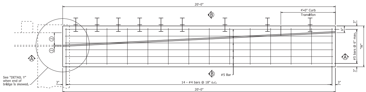
PLAN OF APPROACH GUTTER 3/4" = 1'-0"
