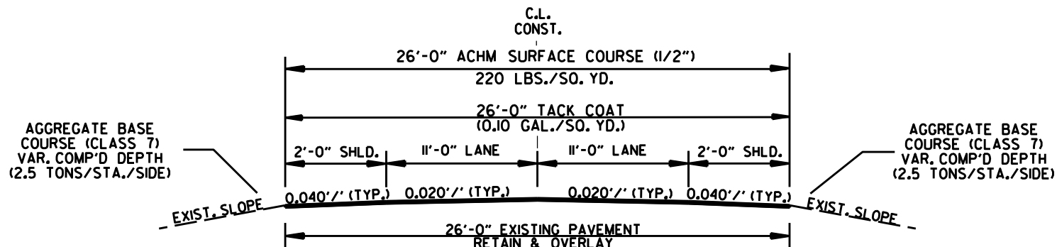
2 LANE OPEN SHOULDER OVERLAY LOG MILE 0.755 TO LOG MILE 1.702
