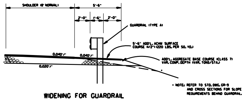
WIDENING FOR GUARDRAIL
