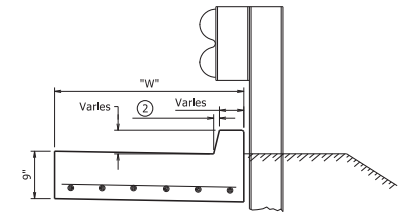
SECTION B-B 1" = 1'-0"
