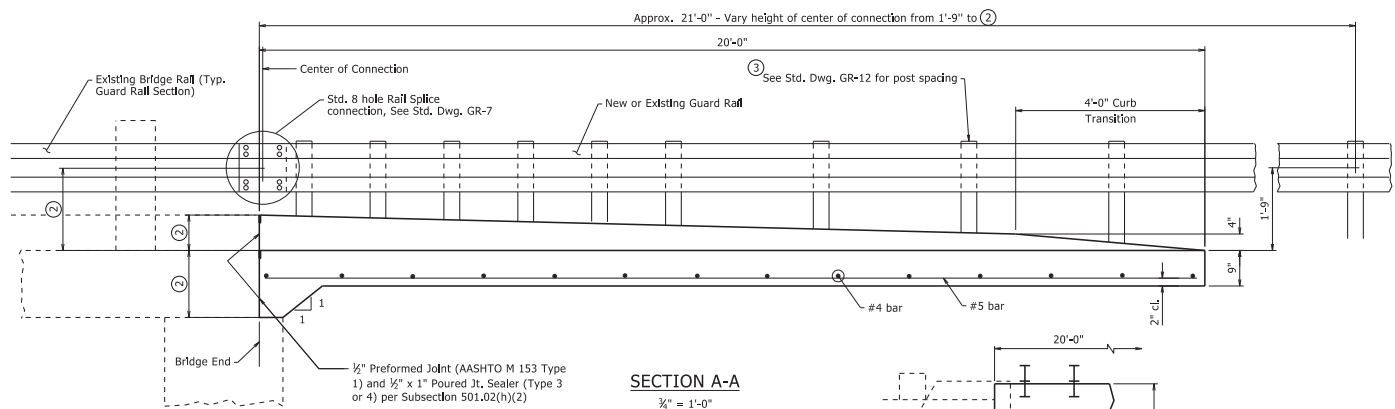
PLAN OF APPROACH GUTTER 3/4" = 1'-0"
