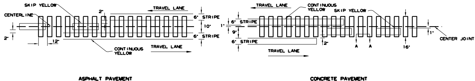
LOCATION PLAN OF CENTERLINE RUMBLE STRIPES
