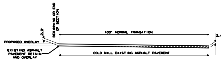
DETAIL FOR TRANSITIONS
