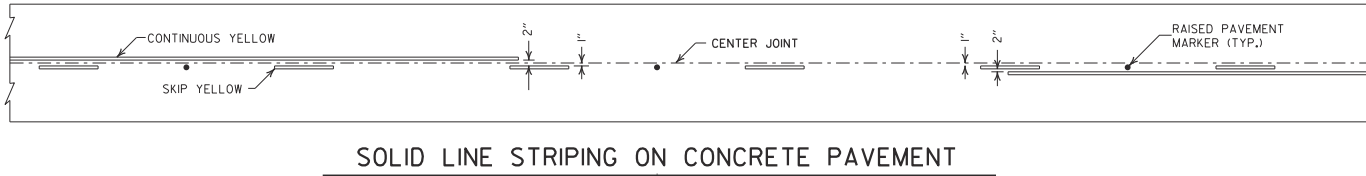
CONCRETE PAVEMENT
