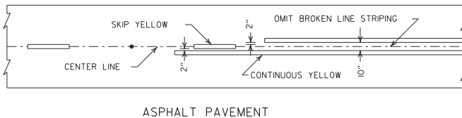
ASPHALT PAVEMENT
