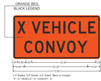
WZ-2 SIGN
