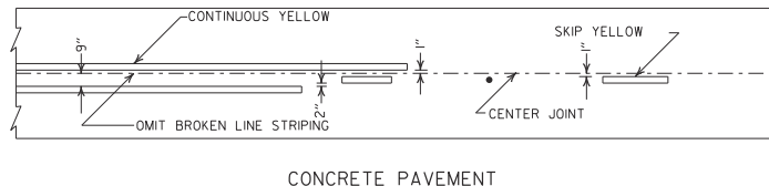
CONCRETE PAVEMENT
