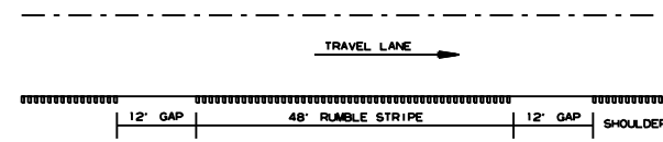
DETAIL FOR GAP PATTERN RUMBLE STRIPE
