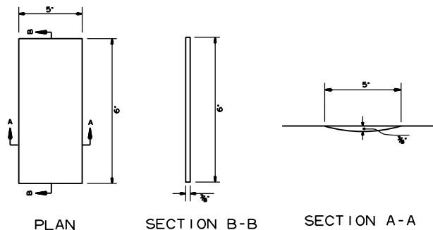
DETAILS OF RUMBLE STRIPE
