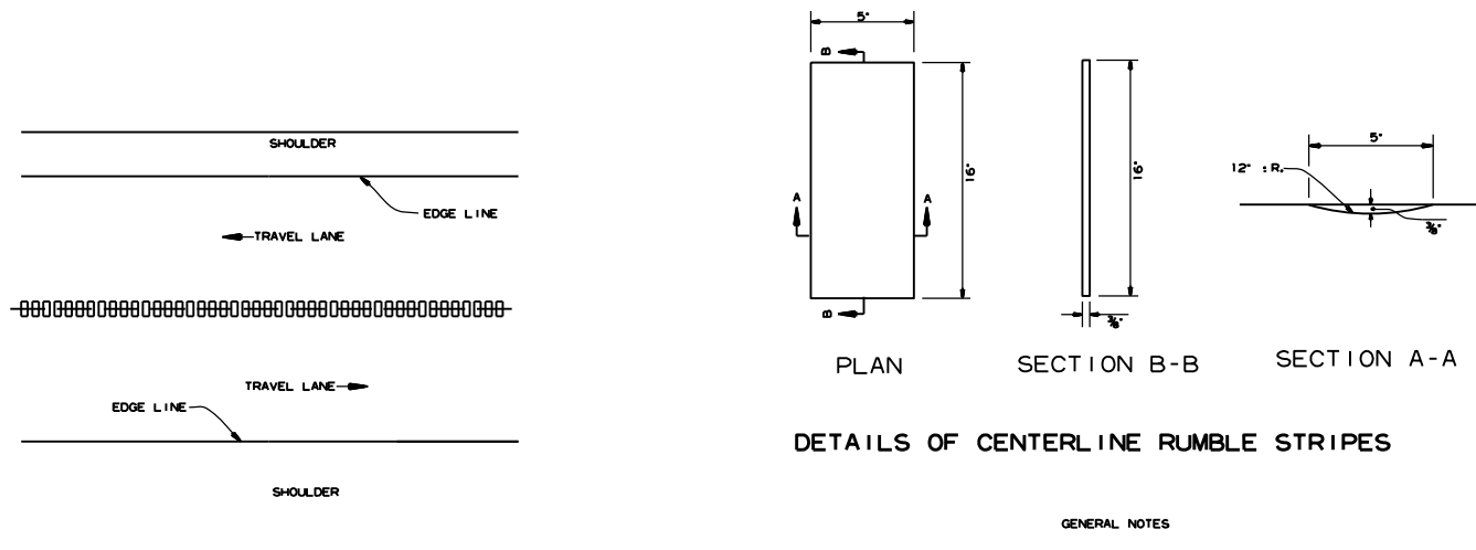
LOCATION PLAN OF CENTERLINE RUMBLE STRIPES
