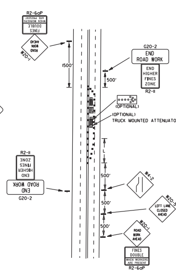
(F) TYPICAL APPLICATION - 4-LANE UNDIVIDED ROADWAY WITH INSIDE LANE CLOSED.
