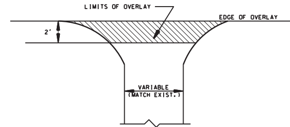
DETAIL FOR DRIVEWAY TURNOUTS (PAVEMENT PRESERVATION)
