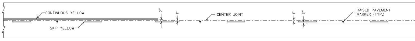
CONCRETE PAVEMENT
