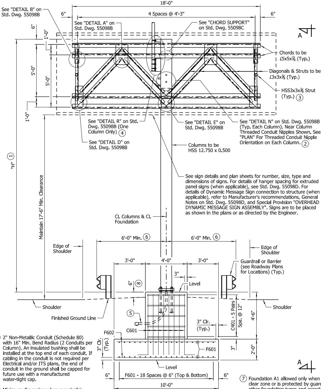
ELEVATION - FOUNDATION A1 No Scale
