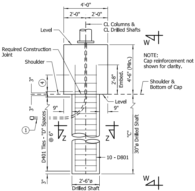
ELEVATION - FOUNDATION B2 ③ Scale: ¾" = 1'-0"
