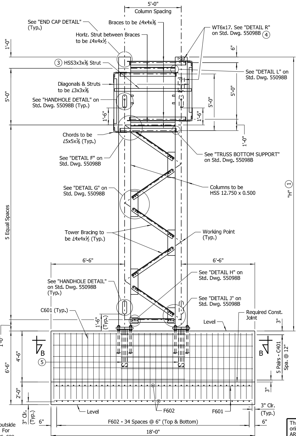
VIEW A-A (Foundation A1) No Scale
