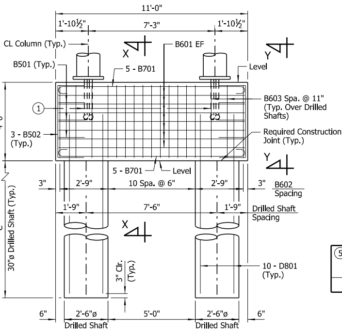
VIEW V-V
