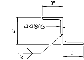
DETAILS OF ALTERNATE Z SUPPORT No Scale
