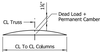
TRUSS CAMBER DIAGRAM
