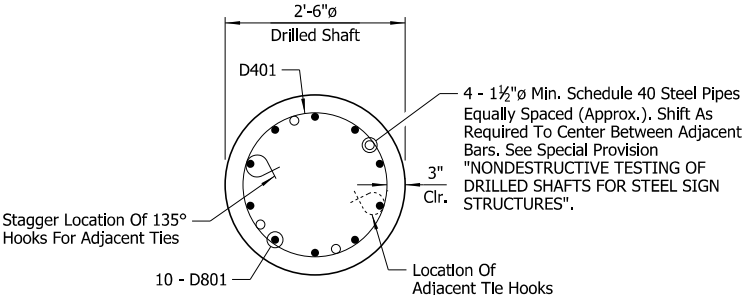
SECTION Z-Z
