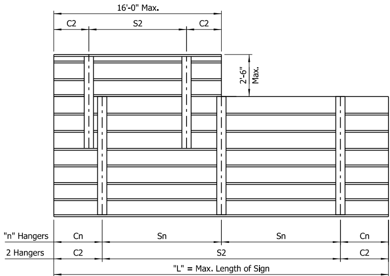
HANGER SPACING DETAILS FOR EXTRUDED PANEL SIGNS No Scale
