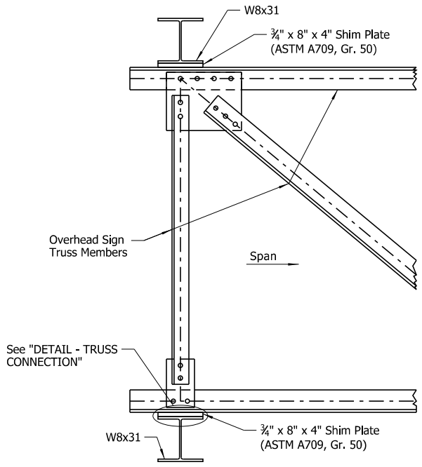
VIEW C-C No Scale
