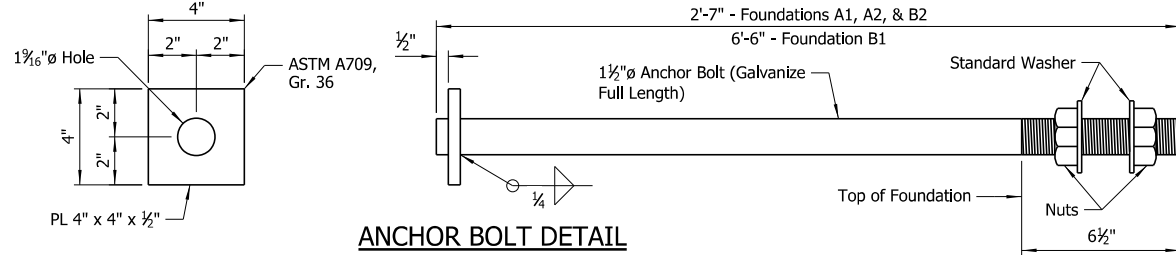
ANCHOR BOLT DETAIL No Scale
