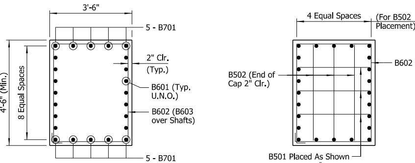
SECTION X-X
