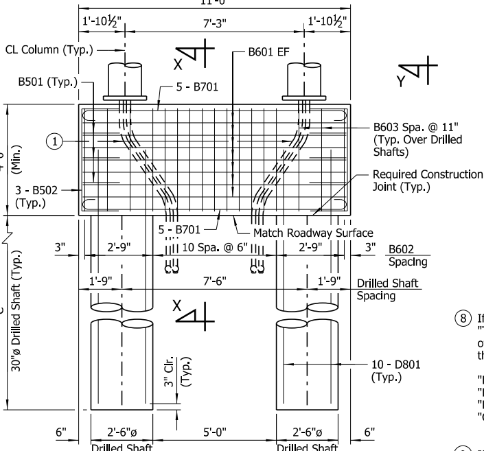
VIEW W-W
