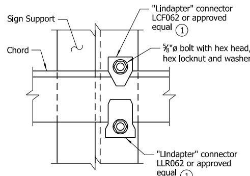
SECTION THRU TRUSS No Scale
