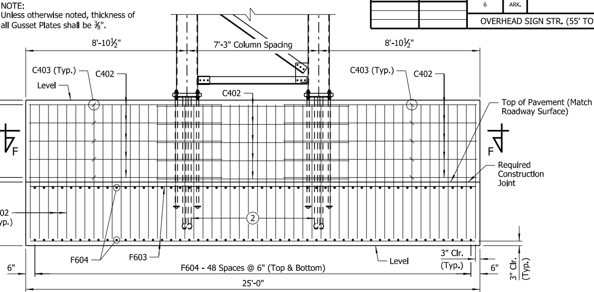
VIEW AA-AA (Foundation B1) Scale: \frac{3}{8} " = 1'-0"
