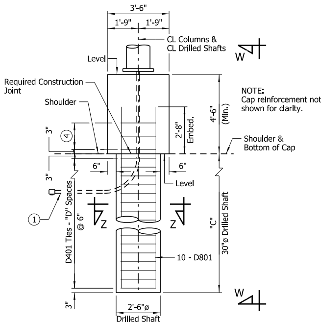
ELEVATION - FOUNDATION B2 ③
