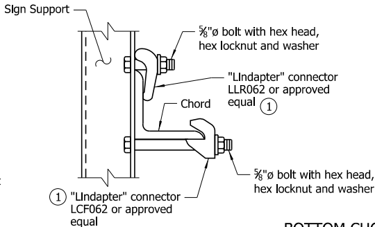
BOTTOM CHORD
