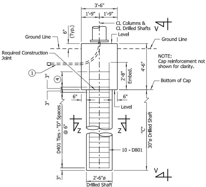
ELEVATION - FOUNDATION A2 ②
