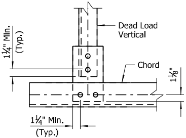
DETAIL G No Scale
