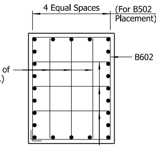
VIEW Y-Y
