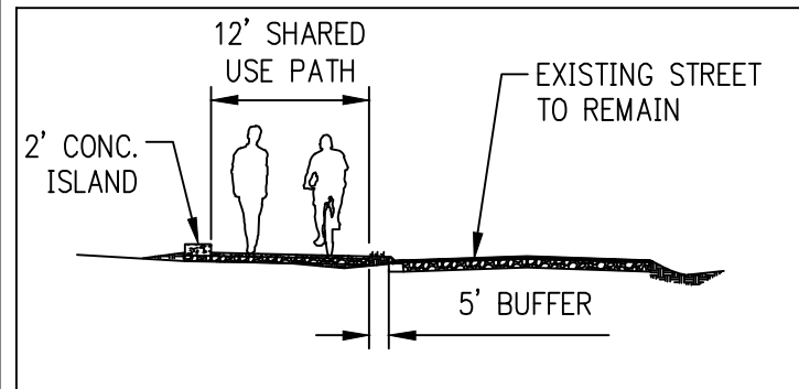
TYPICAL PATH SECTION NTS (FACING NORTH) HIGH ROAD TO SHANNON HILLS DRIVE
