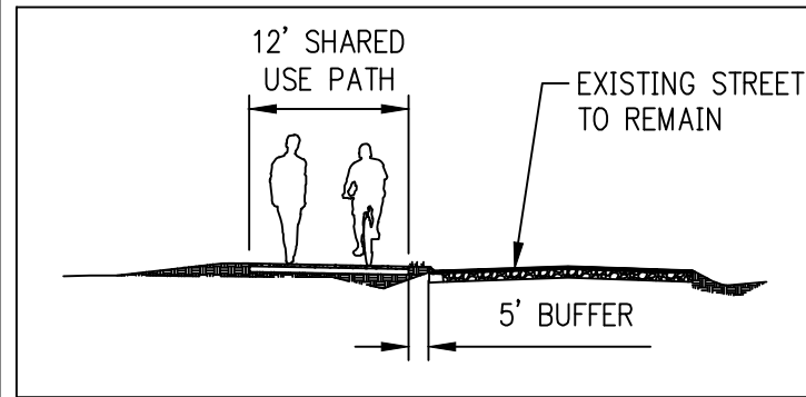
TYPICAL PATH SECTION NTS (FACING NORTH) TALL PINE DRIVE TO HIGH ROAD
