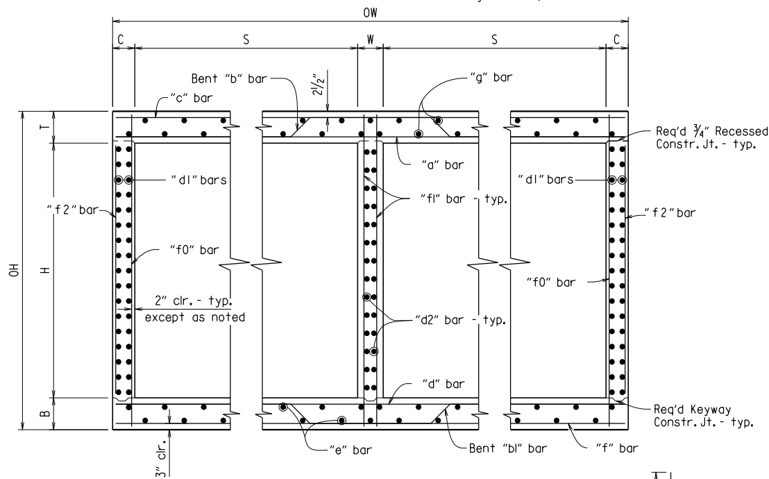
TYPICAL SECTION M-M
