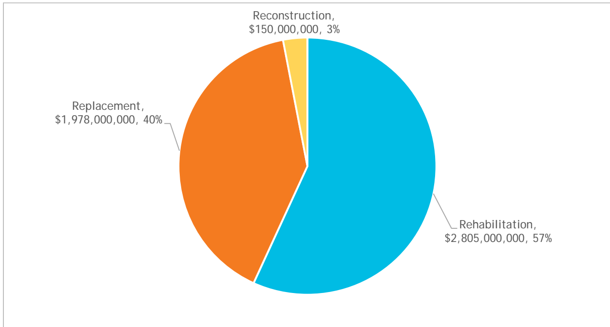
Figure 6.1: State Highway System Bridge Needs, 2016-2040
