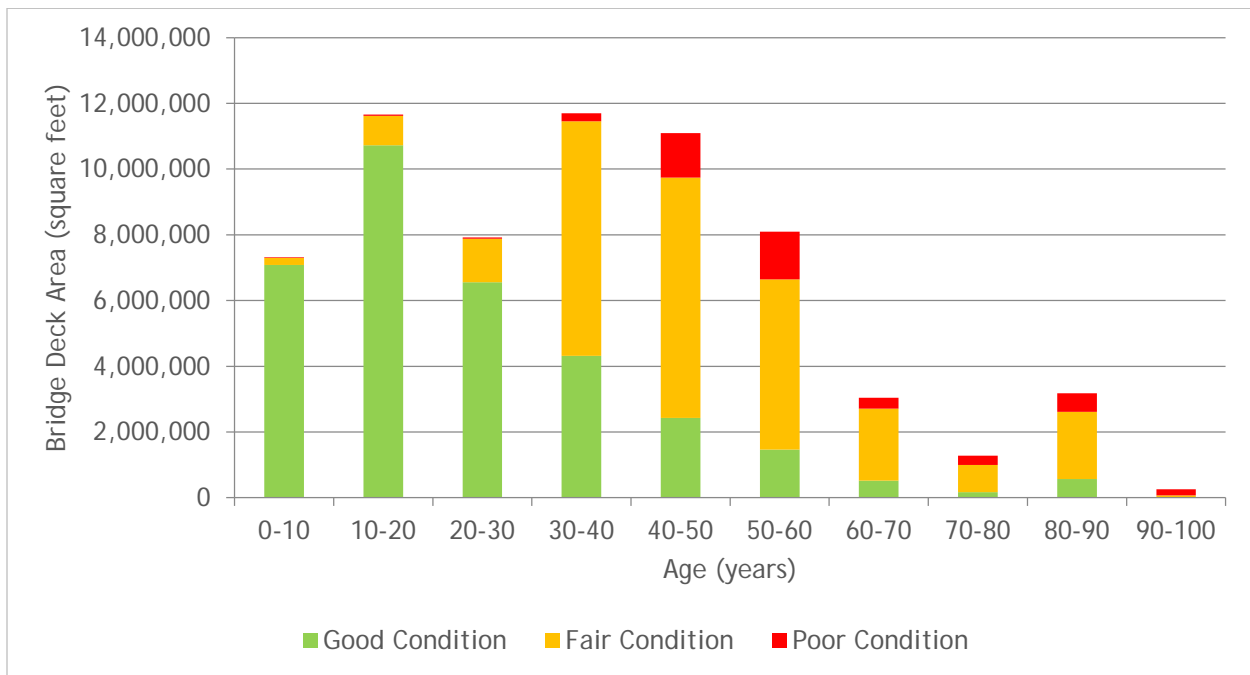
Figure 5.4: Bridge Condition by Age (as of 2015)
