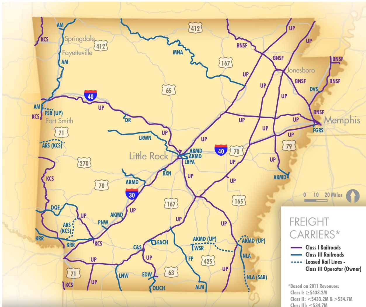
Figure 5.6: Arkansas Freight Rail System
