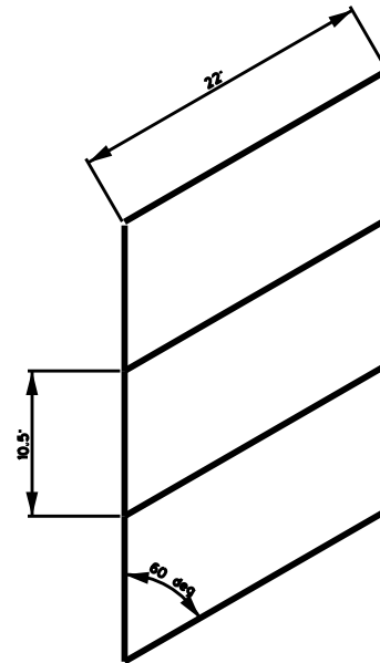
DETAIL FOR PARKING STRIPING STRIPING 4" WIDTH
