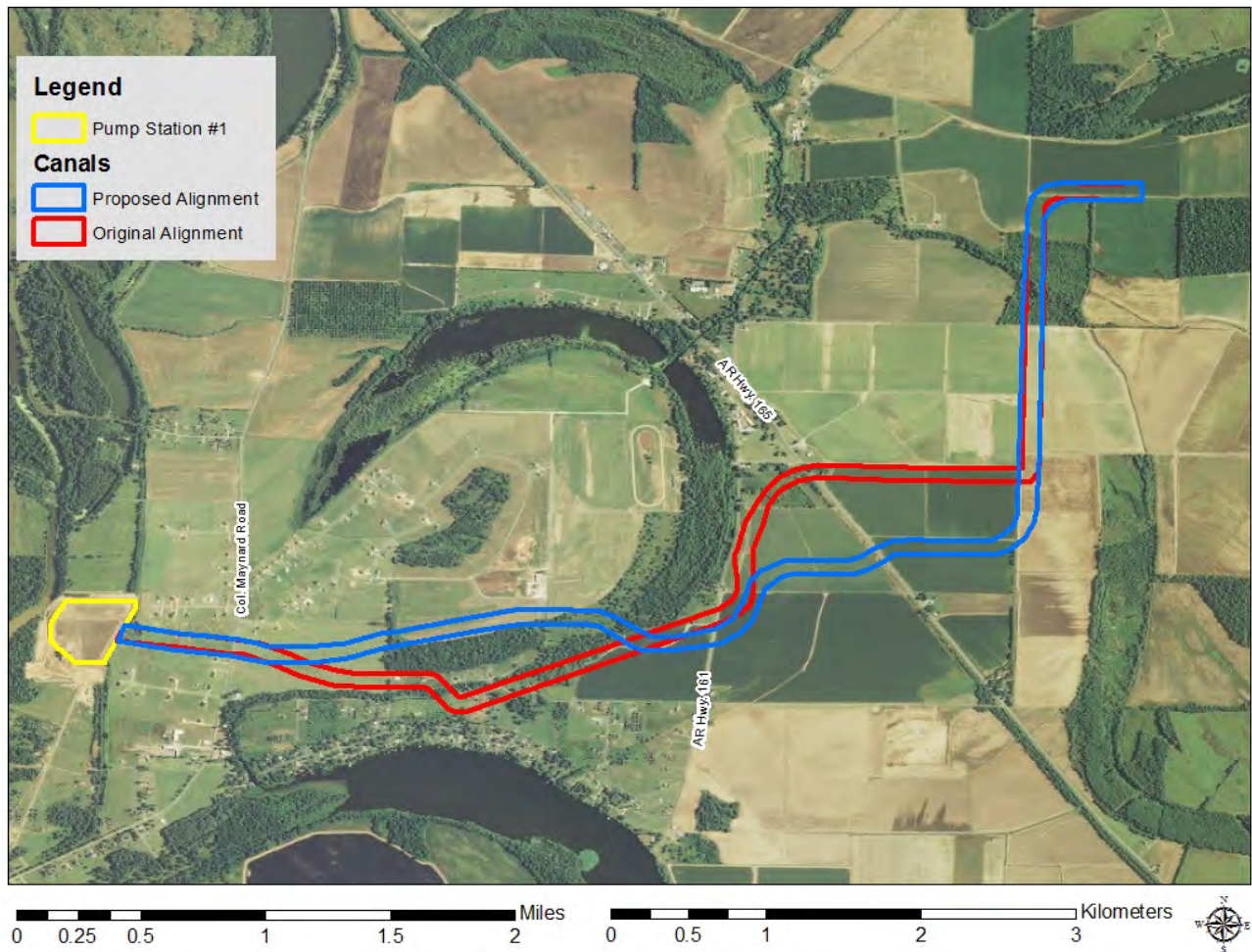
Figure 2. Location of the re-alignment of Canal 1000 near Scott, Arkansas. The proposed modification would save approximately $2,900,000 by avoiding a bridge demolition and construction of an additional bridge over Scott Bayou.
