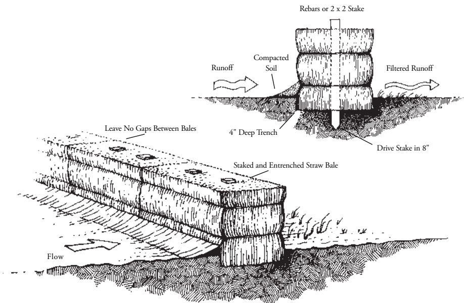
Figure 11.1 Straw bale fencing to slow runoff and trap sediment for sheet flow or channelized flow.
