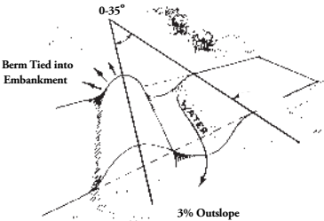
Water Bar Installation
